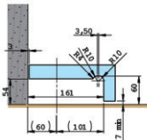
GFS-20 Bottom Patch
