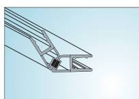
GPS-M3 Magnetic Seal 135° 08mm (2.2mtr) - ₹ 925/- 10mm (2.2mtr) - ₹ 925/- 12mm (2.2mtr) - ₹ 1100/- 10mm (2.5mtr) - ₹ 1100/- 12mm (2.5mtr) - ₹ 1300/-
